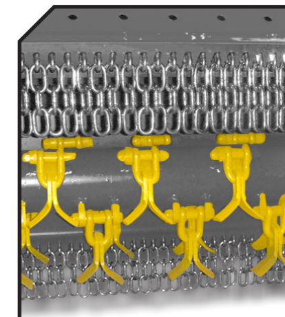
Rotor with grass flails or forged hammers
