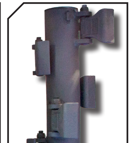
Rotor with grass flails or forged hammers
